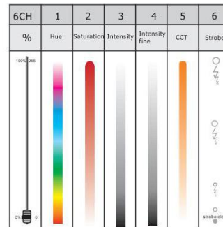
VG-PL100G DMX Channel
