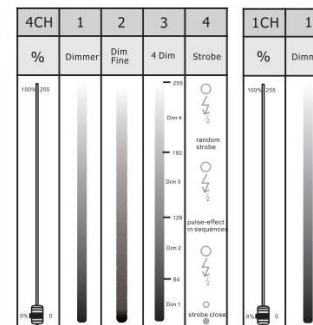
VG-PL100W DMX Channel
